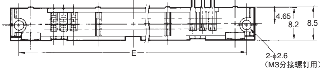
(DIP直端子)
